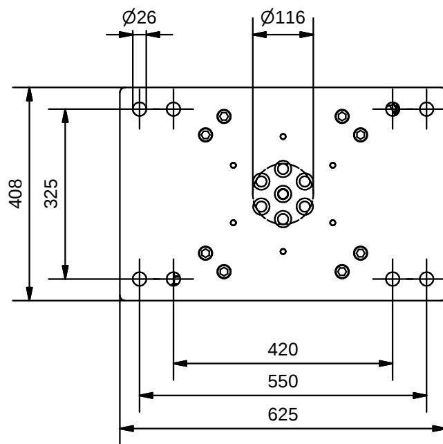
Bottom view (1:10)
